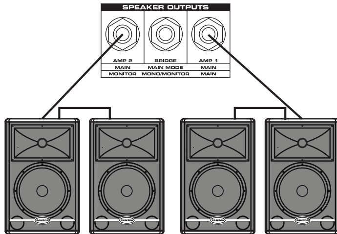
When connecting two speakers to AMP 1 and two speaker to AMP 2, use speakers with an 8–16 Ohm impedance rating.
