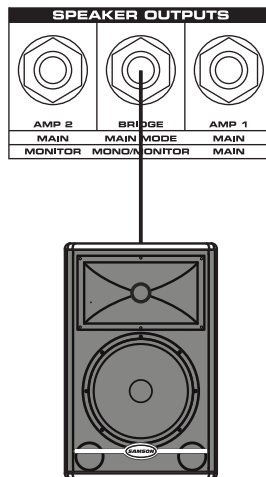
When the POWER AMPS are in BRIDGE mode, use a speaker with an 8–16 Ohm impedance rating.
