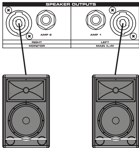
When connecting one speaker to AMP1 and one speaker to AMP 2, use speakers with a 4–8 Ohm impedance rating.
