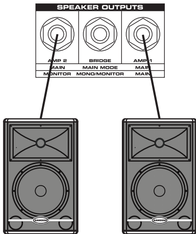
When connecting one speaker to AMP1 and one speaker to AMP 2, use speakers with a 4–8 Ohm impedance rating.
